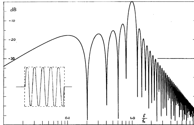
Fig. 1. Spectrum of a five-cycle tone burst of frequency f_0 . The high-frequency rolloff approaches 12 dB/octave, but only 6 dB/octave for the low frequencies. JOURNAL OF THE AUDIO ENGINEERING SOCIETY, 1980 APRIL, VOLUME 28, NUMBER 4
