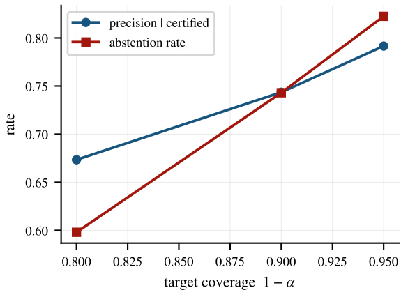
Cost of the certificate
