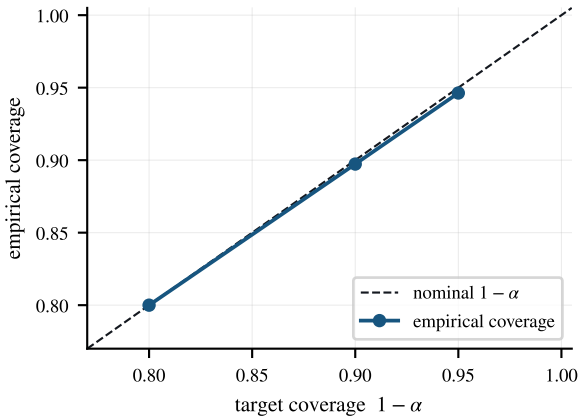
Theorem 7: marginal coverage
