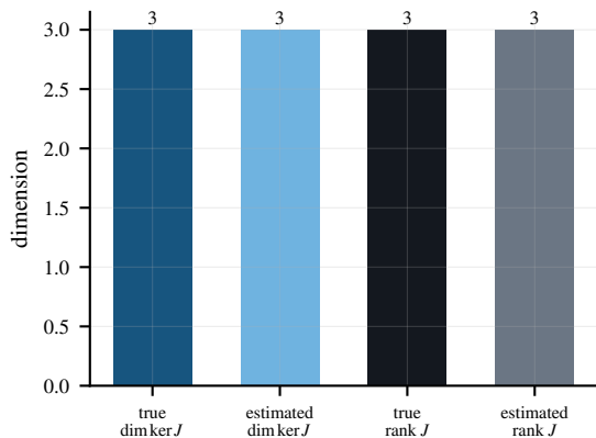
Recovered dimensions ( d_X = 6 )
