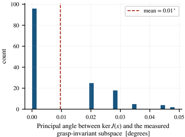
Theorem 4 verified at 50 states
