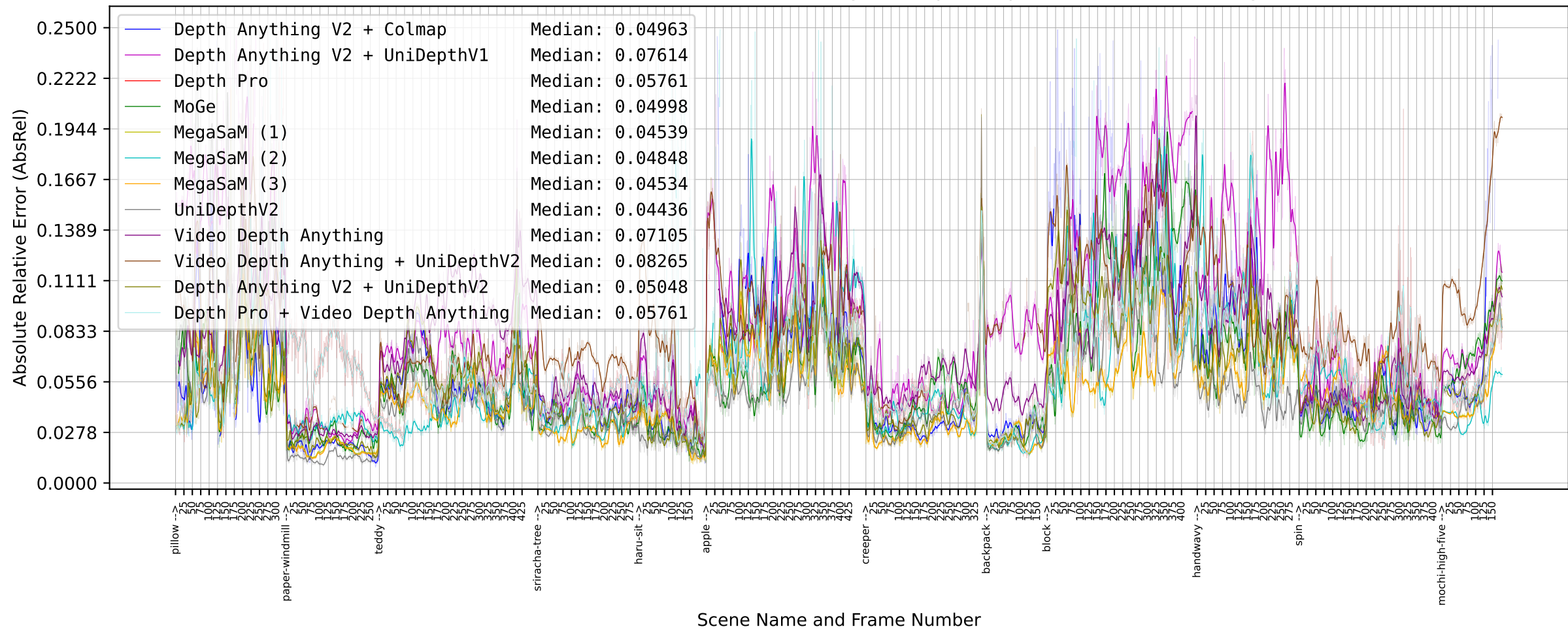
Absolute Relative Error (AbsRel) of Lidar aligned Depth Mapsvs. Lidar (Whole Image)
