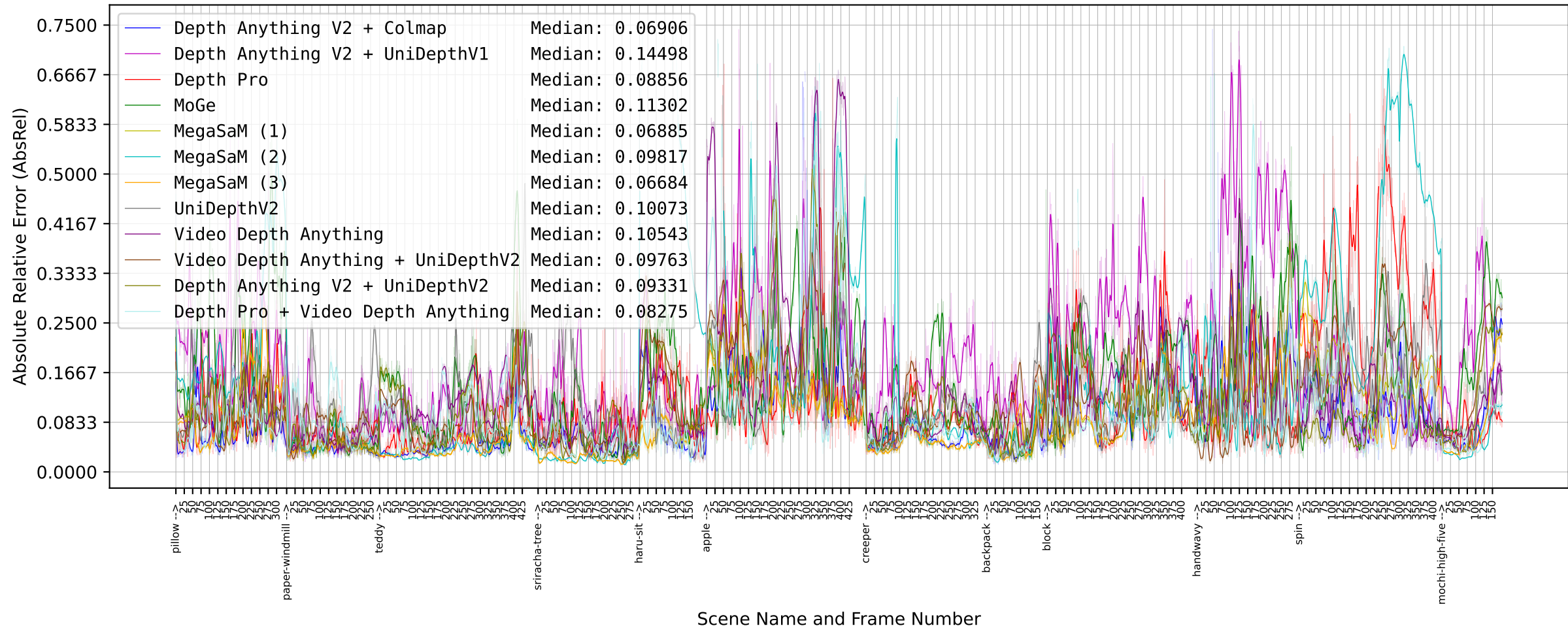
Absolute Relative Error (AbsRel) of Lidar aligned Depth Maps (via RANSAC) vs. Lidar (Foreground)
