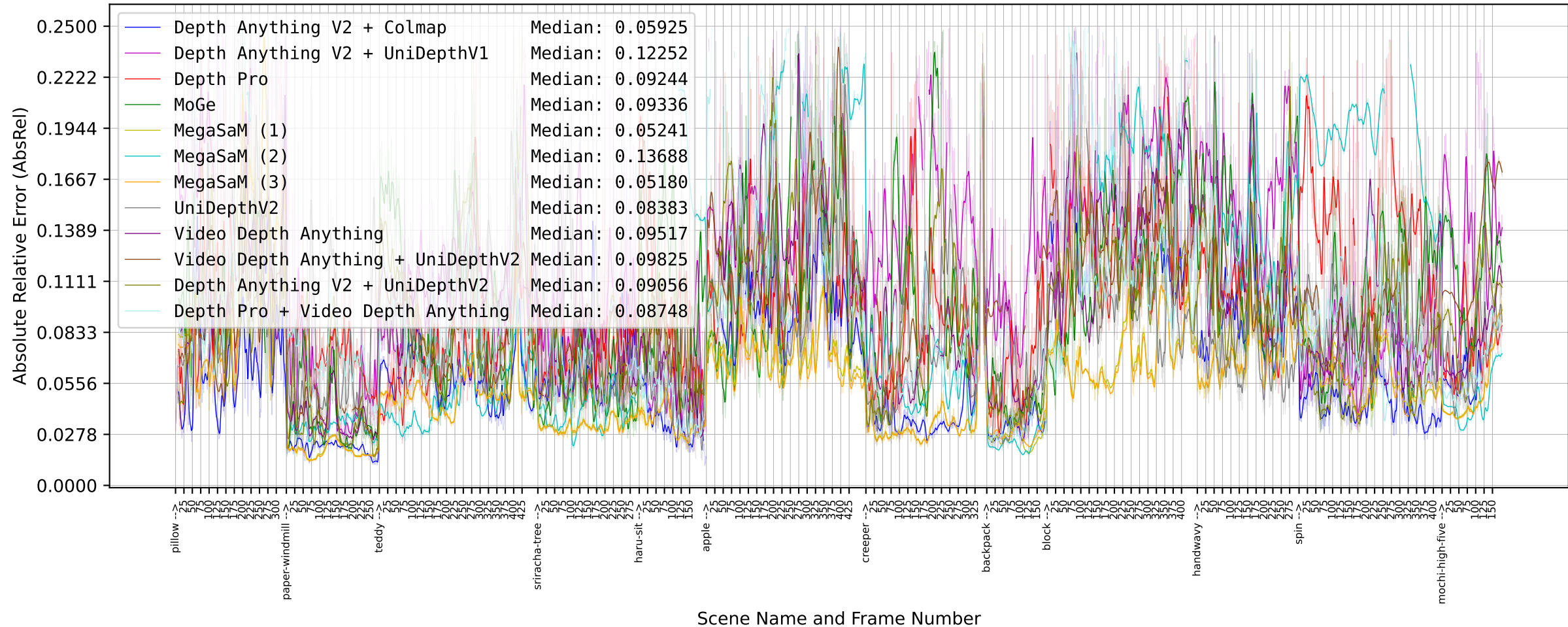
Absolute Relative Error (AbsRel) of Lidar aligned Depth Maps (via RANSAC) vs. Lidar (Whole Image)
