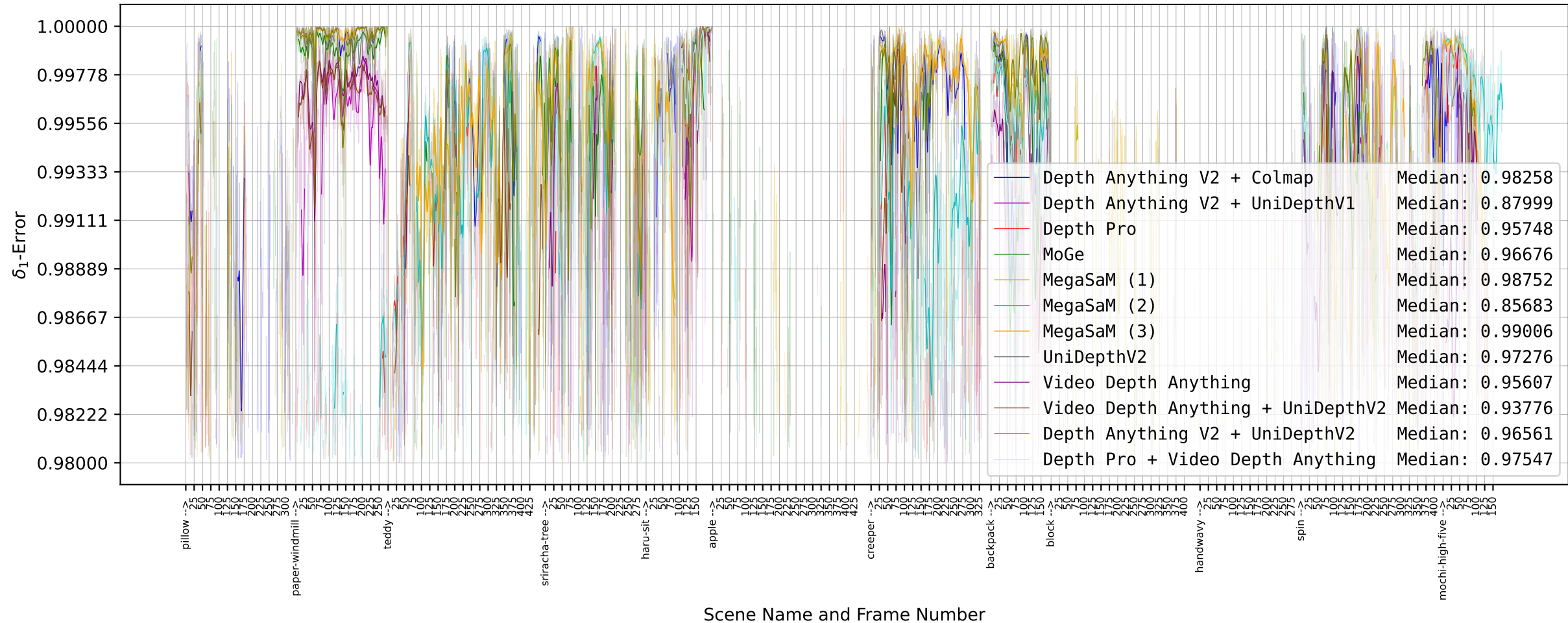
\delta_1 -Error of Lidar aligned Depth Maps (via RANSAC) vs. Lidar (Whole Image)
