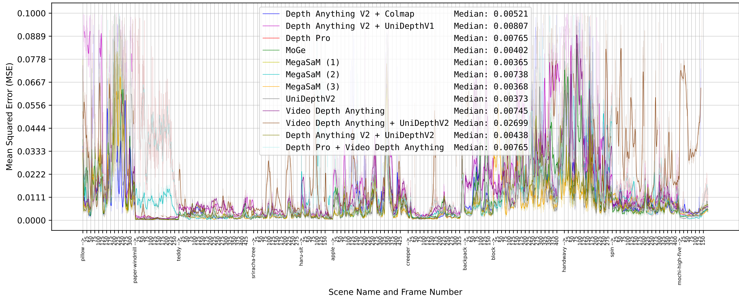
Mean Squared Error (MSE) of Lidar aligned Depth Maps vs. Lidar (Smoothed + Raw - Whole Image)
