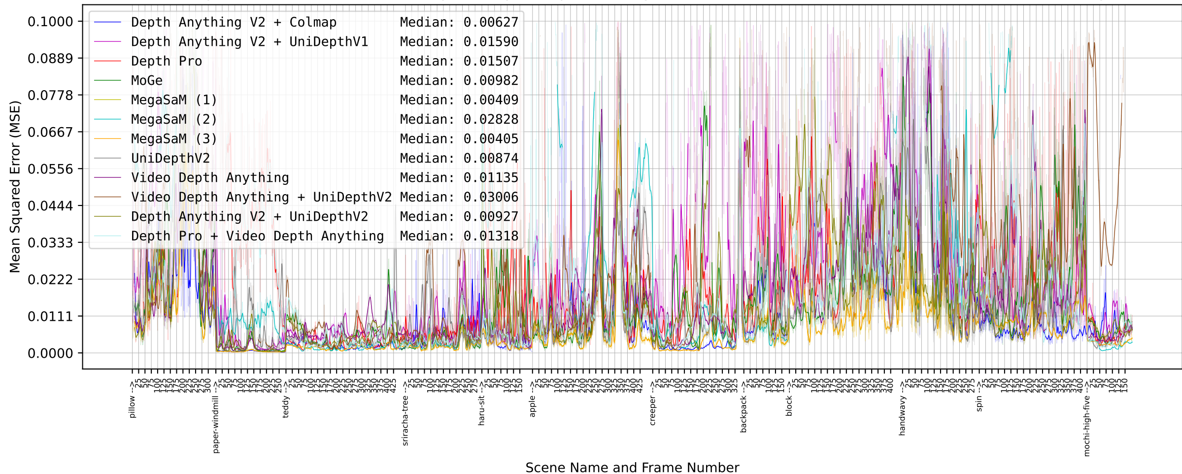
Mean Squared Error (MSE) of Lidar aligned Depth Maps (via avg scale and shift) vs. Lidar (Smoothed + Raw - Whole Image)
