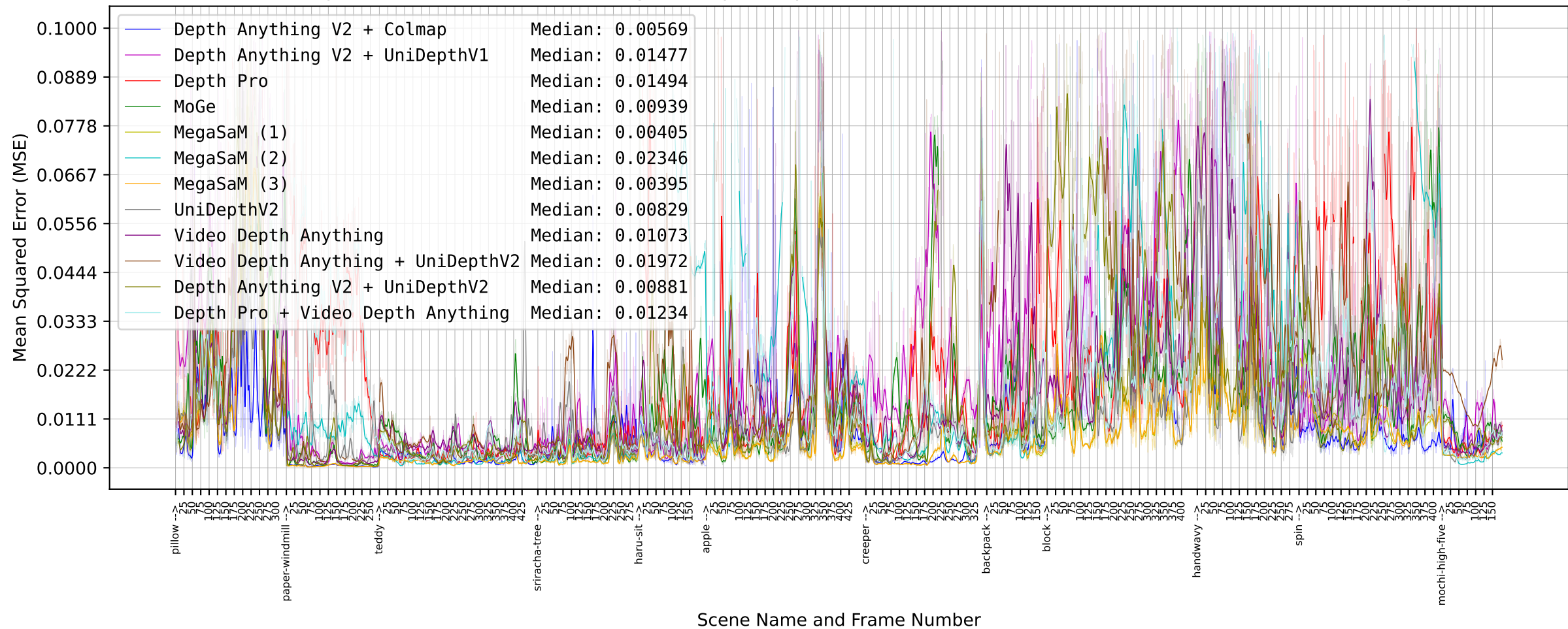
Mean Squared Error (MSE) of Lidar aligned Depth Maps (via RANSAC) vs. Lidar (Smoothed + Raw - Whole Image)
