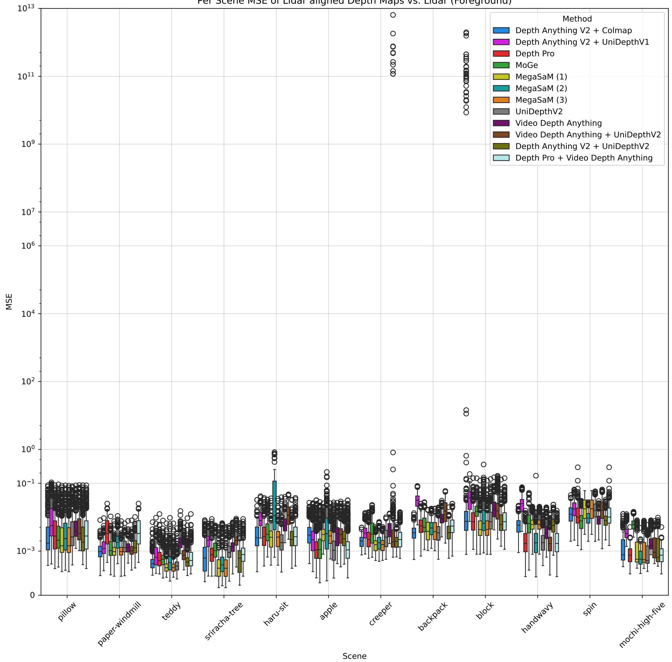
Per Scene MSE of Lidar aligned Depth Maps vs. Lidar (Foreground)
