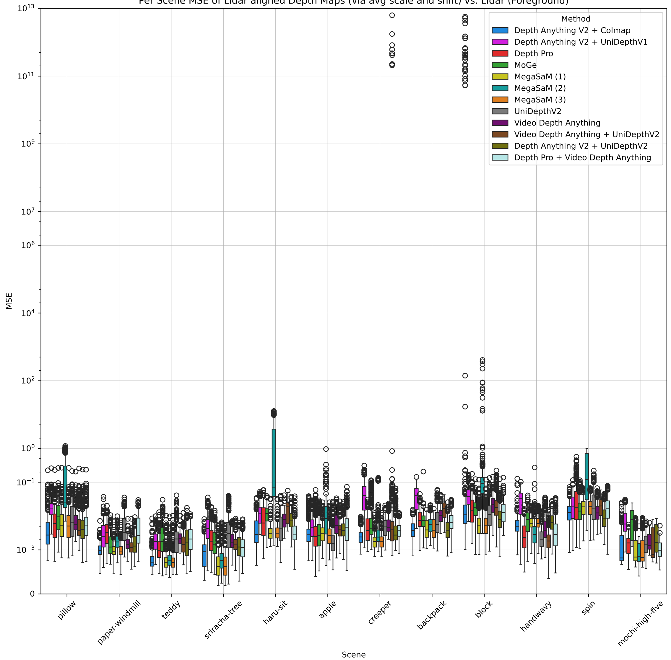
Per Scene MSE of Lidar aligned Depth Maps (via avg scale and shift) vs. Lidar (Foreground)
