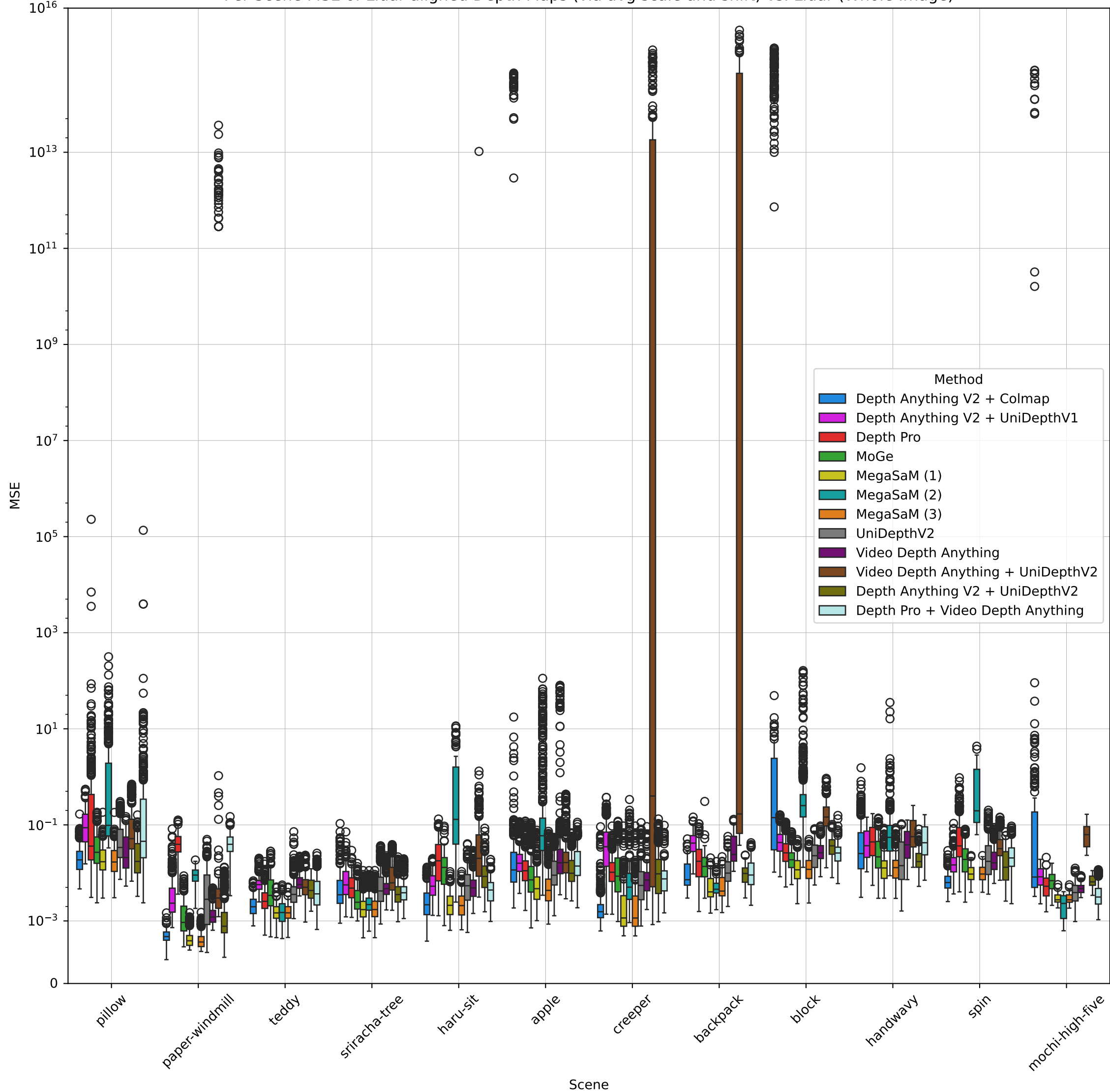
Per Scene MSE of Lidar aligned Depth Maps (via avg scale and shift) vs. Lidar (Whole Image)
