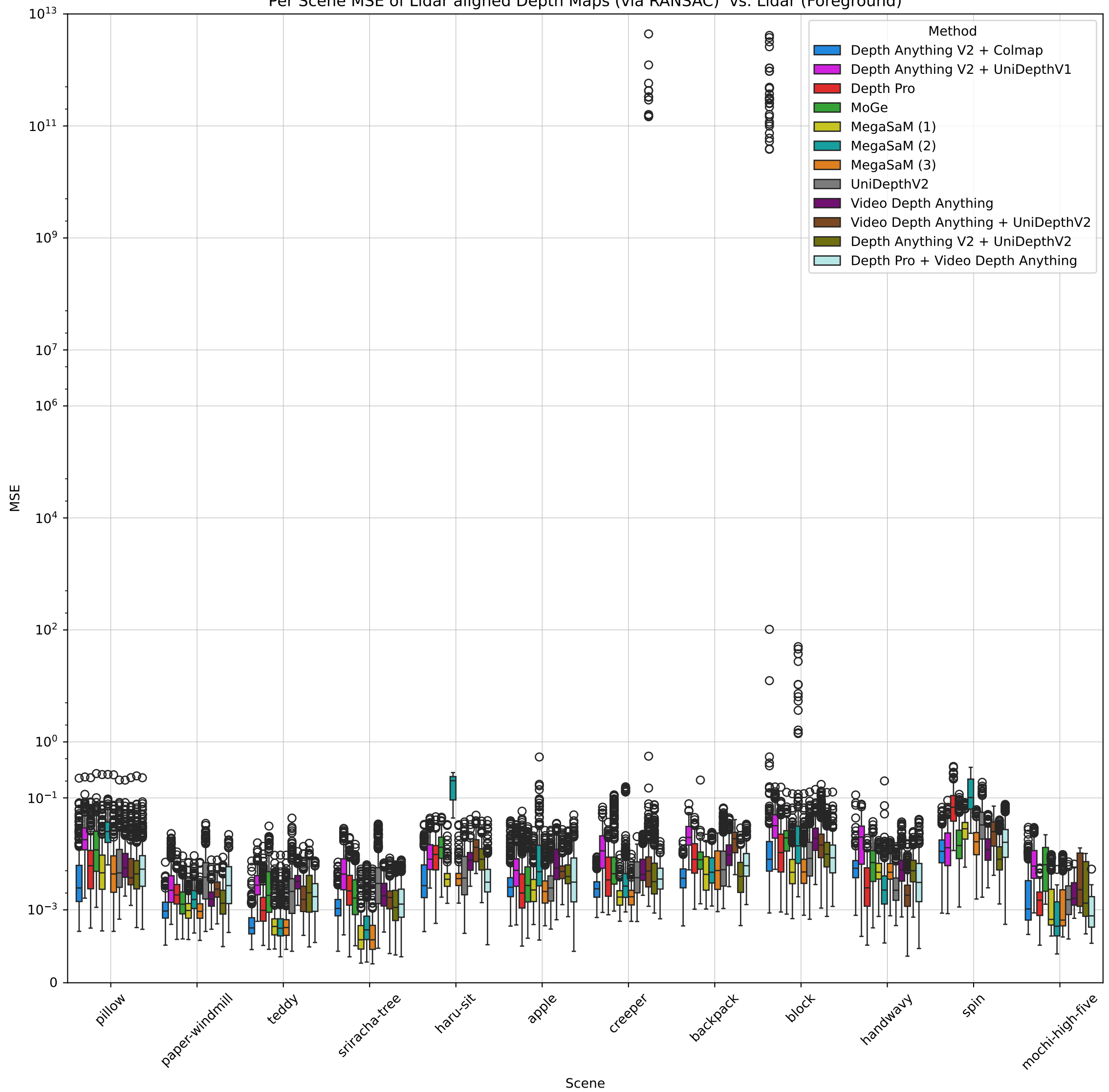
Per Scene MSE of Lidar aligned Depth Maps (via RANSAC) vs. Lidar (Foreground)
