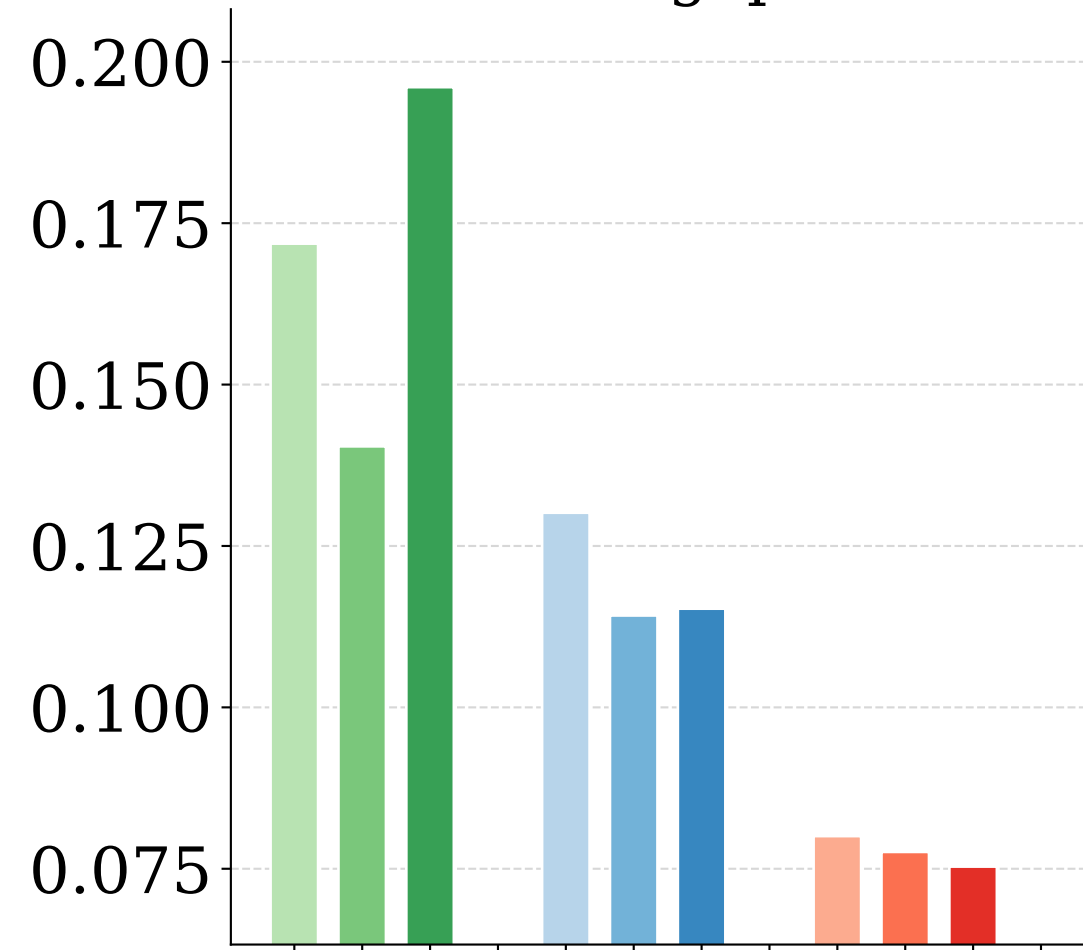
SSIM-gap ↓
