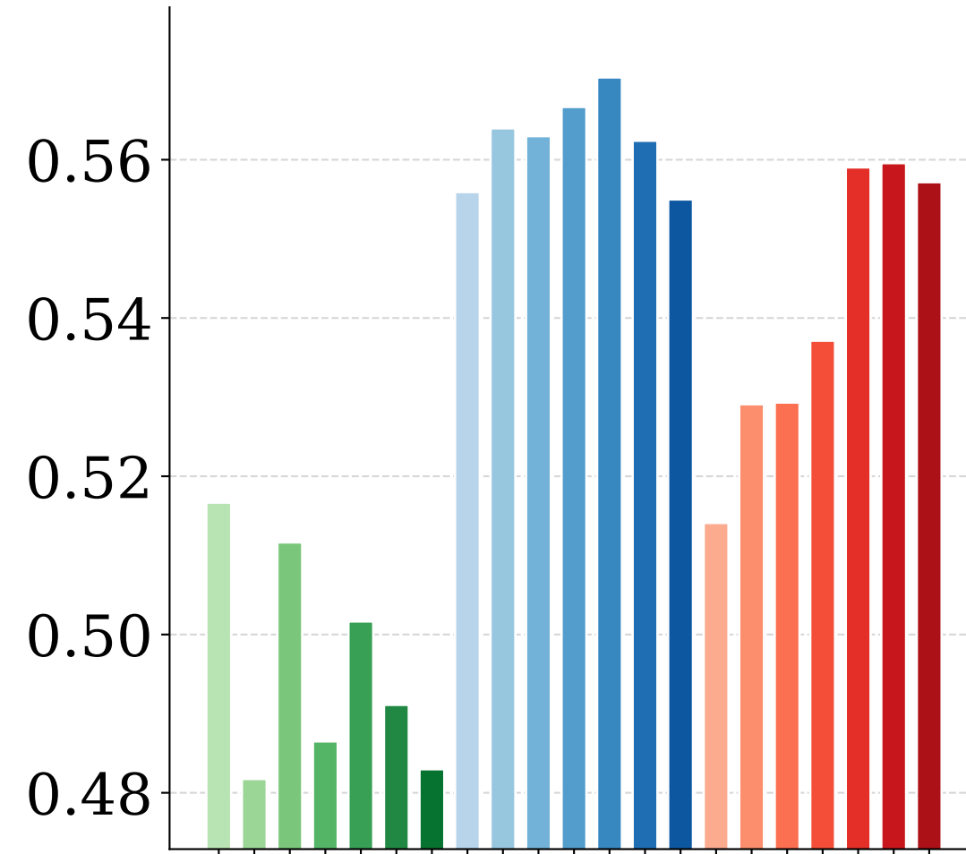
MS-SSIM \uparrow
