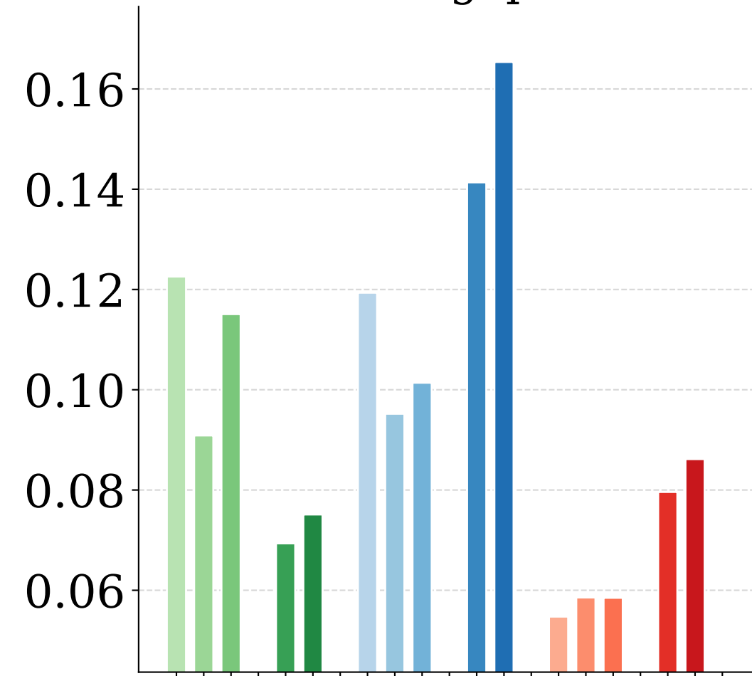
SSIM-gap ↓
