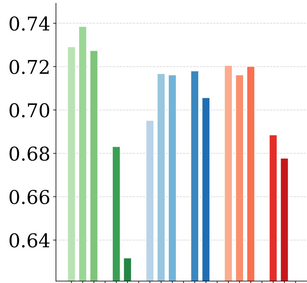
MS-SSIM \uparrow
