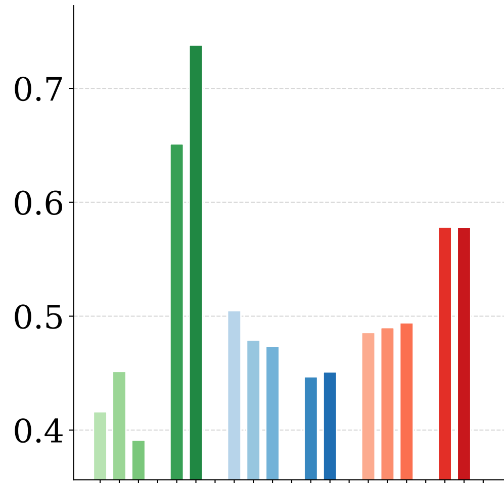
LPIPS \downarrow
