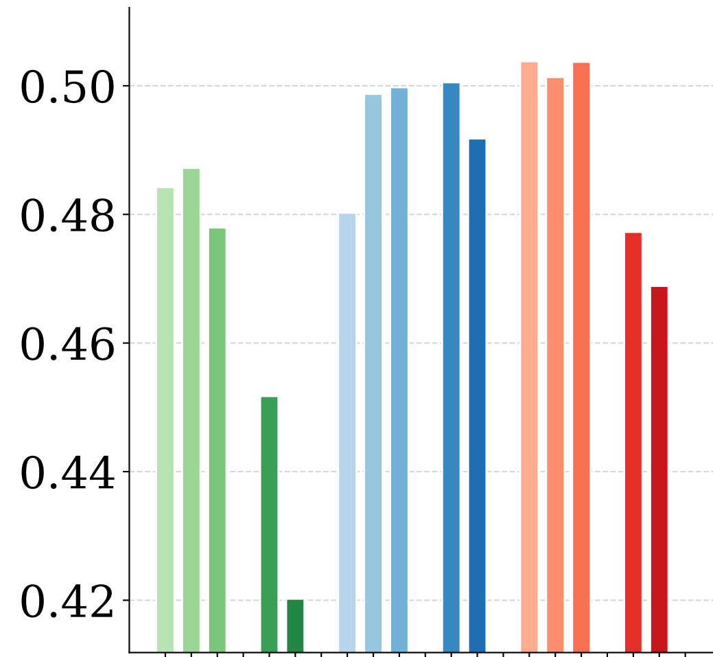
SSIM \uparrow
