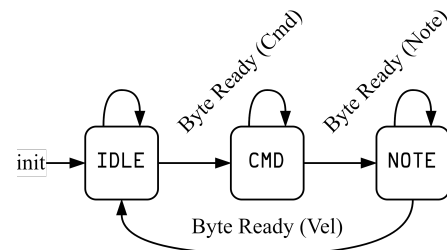
Figure 12: MIDI decoder statemachine
