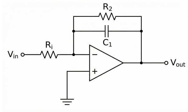
Figure 5: Integrator circuit.
