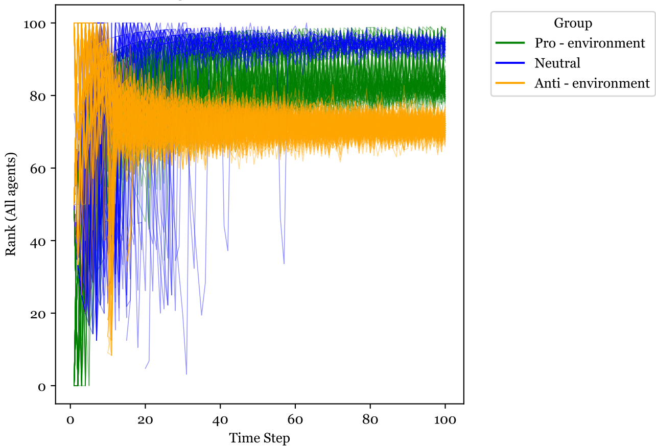
All Agents' Own Rank Over Time
