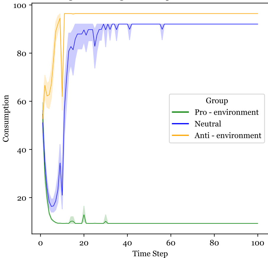
Agents' Average Consumptions Over Time
