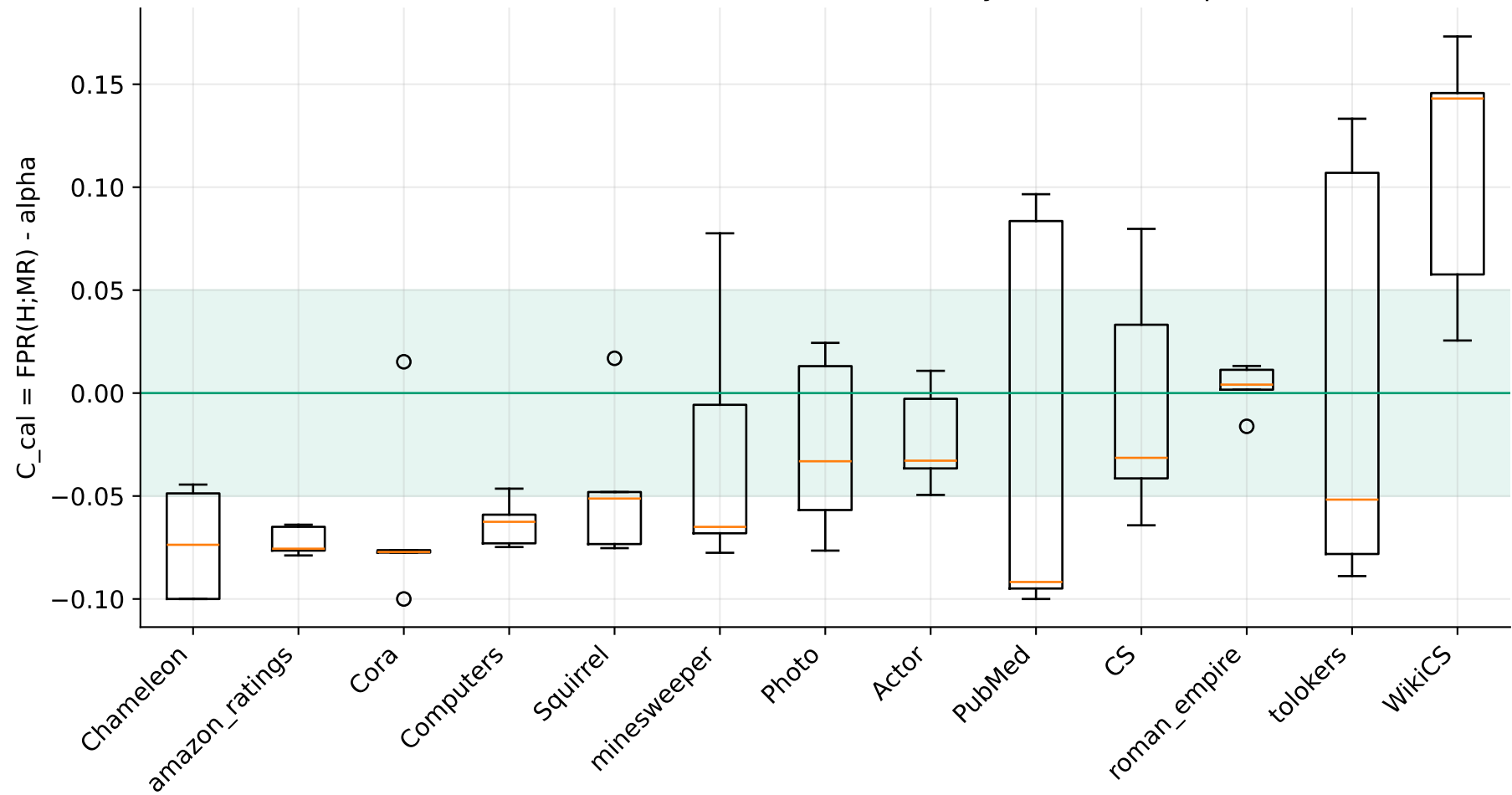
Calibration transfer to the removed client, by dataset (0 = perfect)
