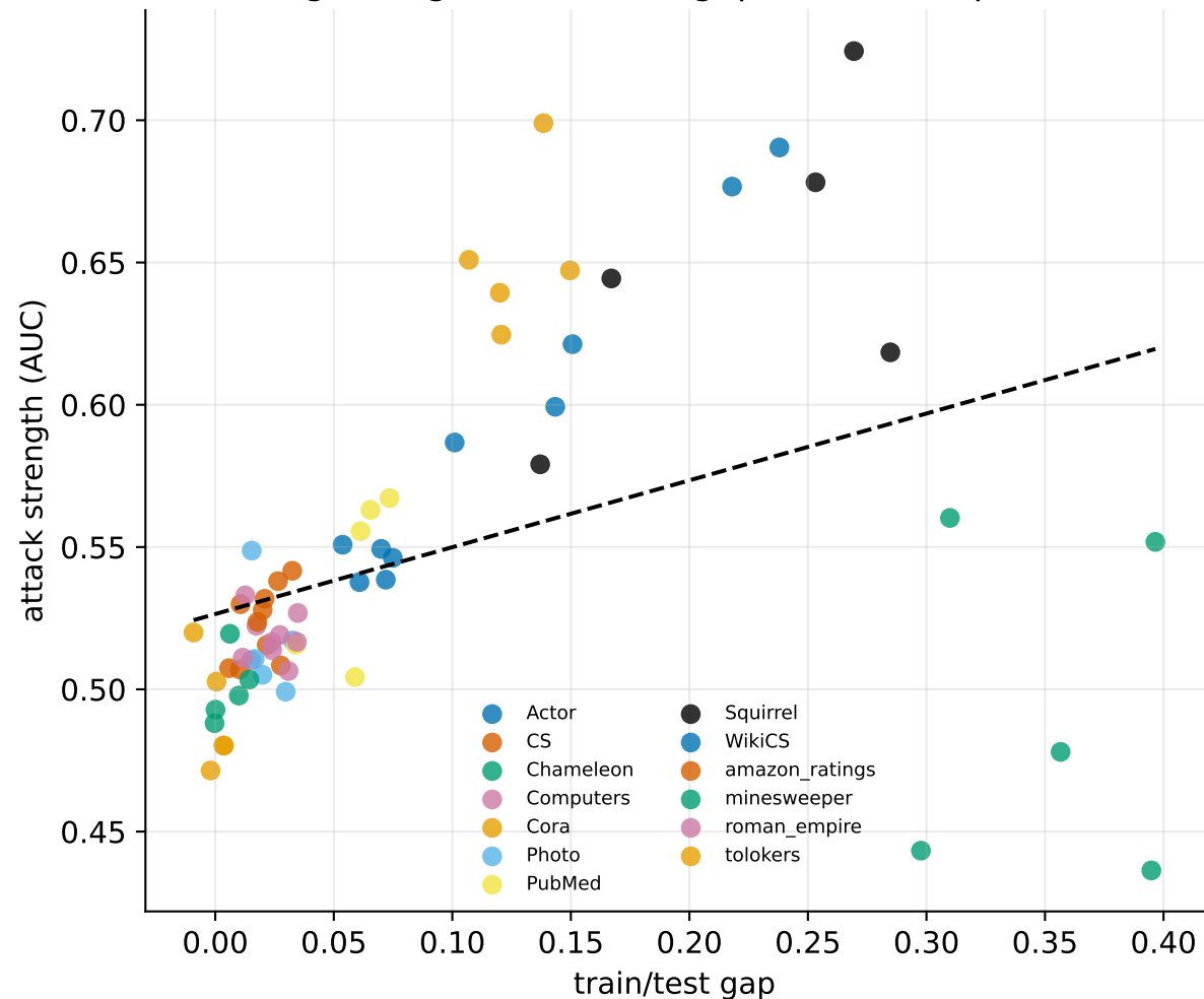
Attack strength vs generalization gap ( r=+0.39 , p=0.001 , n=65 )
