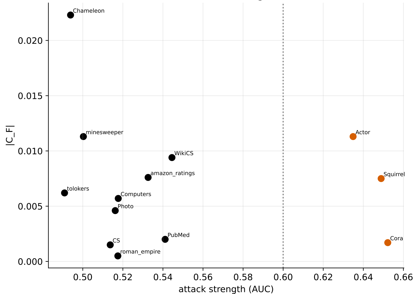
Informative datasets (AUC \geq 0.60, orange) vs weak-attack datasets
