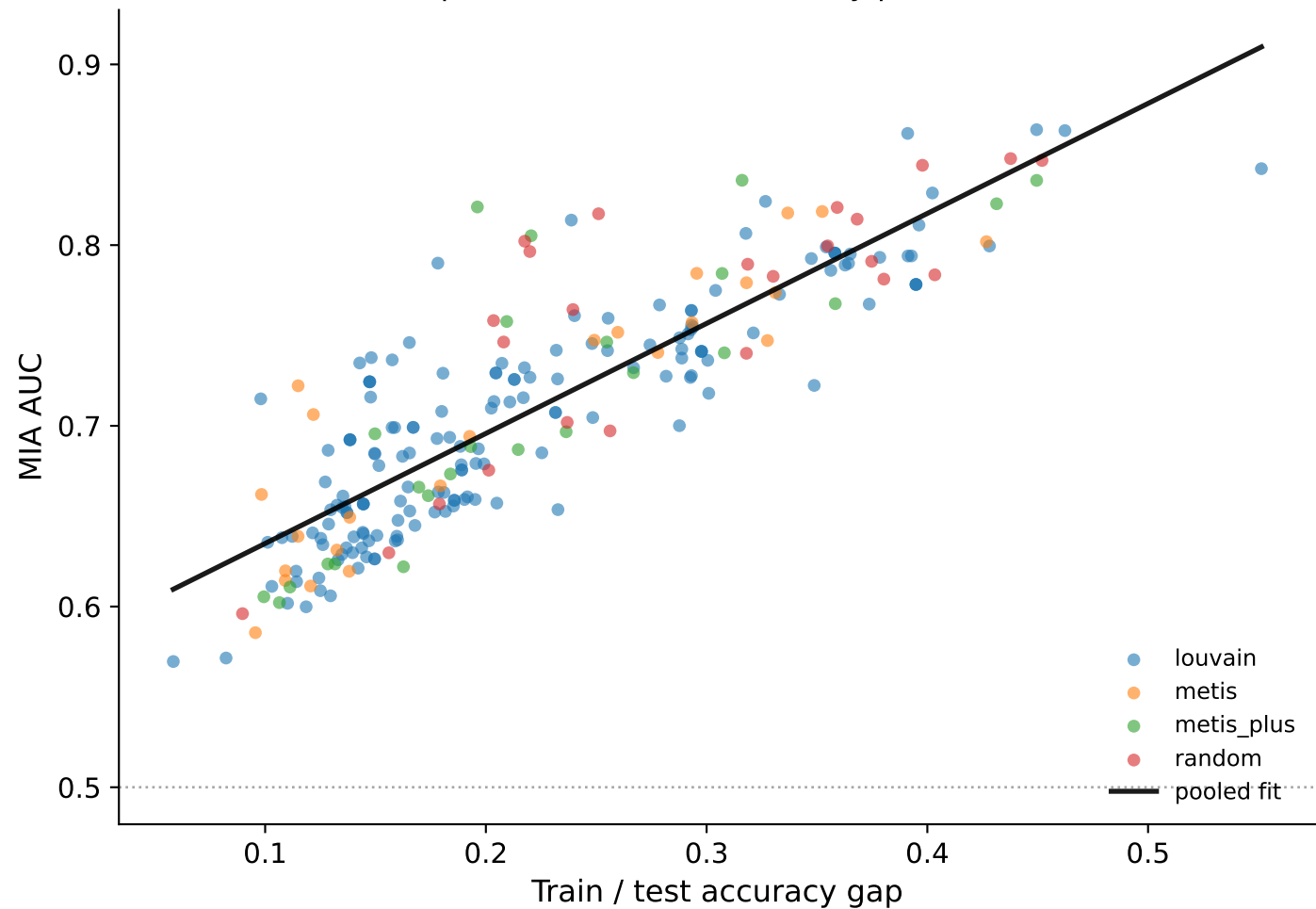
Gap vs MIA AUC — coloured by partitioner
