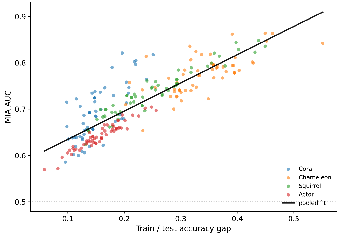
Gap vs MIA AUC — coloured by dataset
