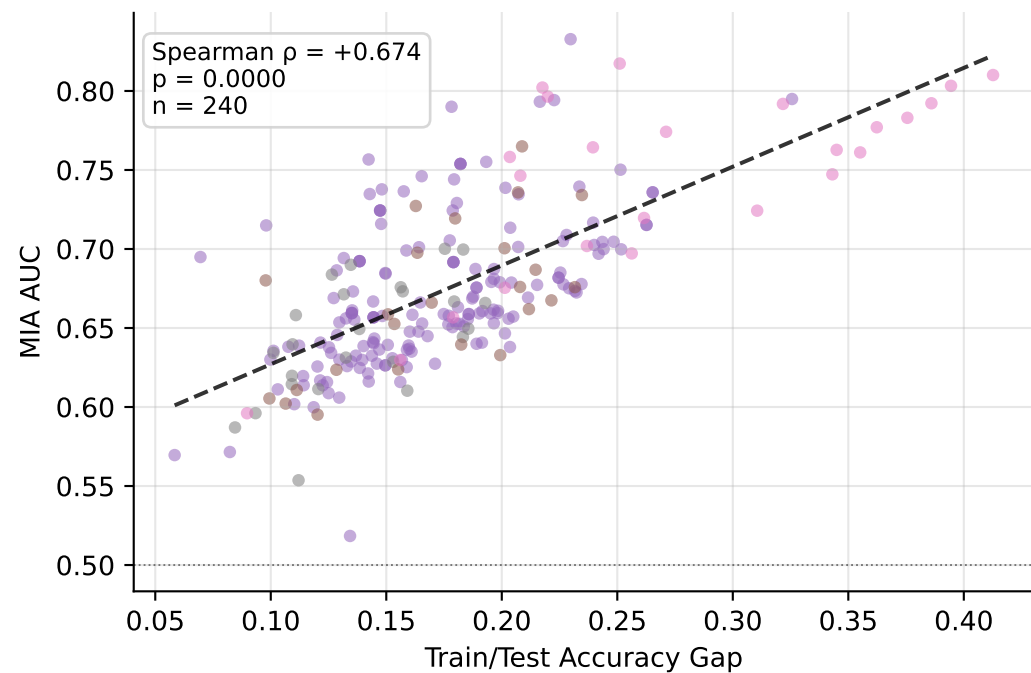
MIA AUC vs. Candidate Predictors (n = 240 across sweep configs)
