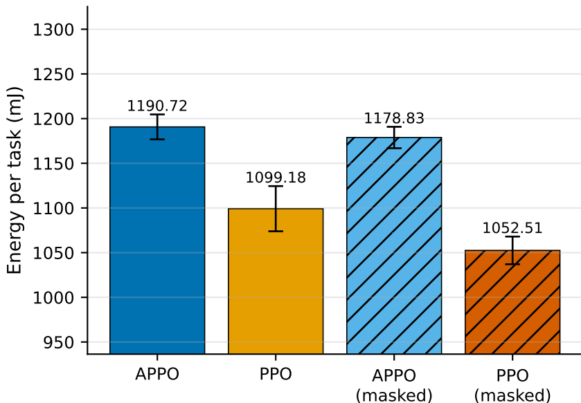
Energy per task (episodes 751-800)
