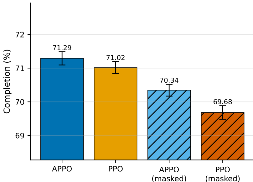
Overall task completion (episodes 751-800)
