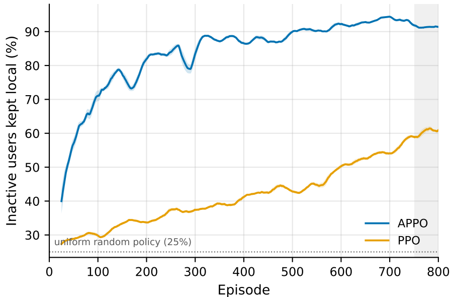
Inactive-user action correctness (unmasked runs)
