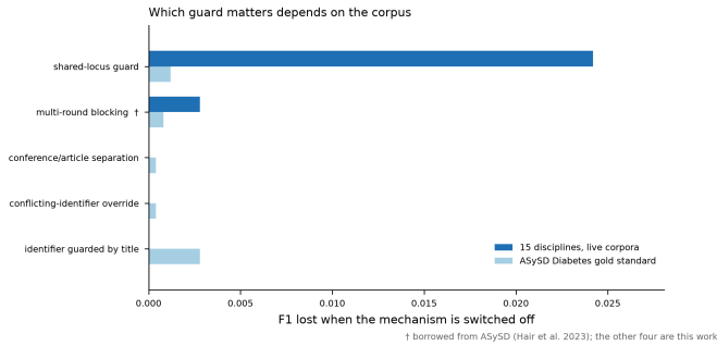
Figure 1: Contribution of each deduplication mechanism, measured by switching it off and rescore. Bars are F1 lost. Multi-round blocking is borrowed from ASySD; the other four are contributed here. The ranking inverts between the two corpora, which is the argument for validating on more than one benchmark.
