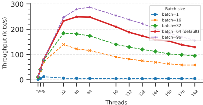
TPC-C throughput vs thread count
