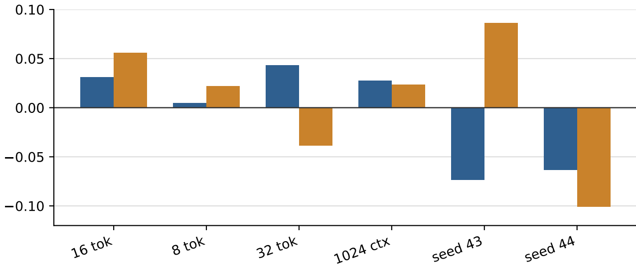
Pearson delta
