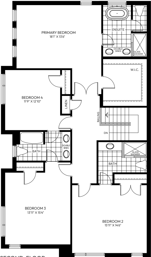
SECOND FLOOR ELEVATION B
