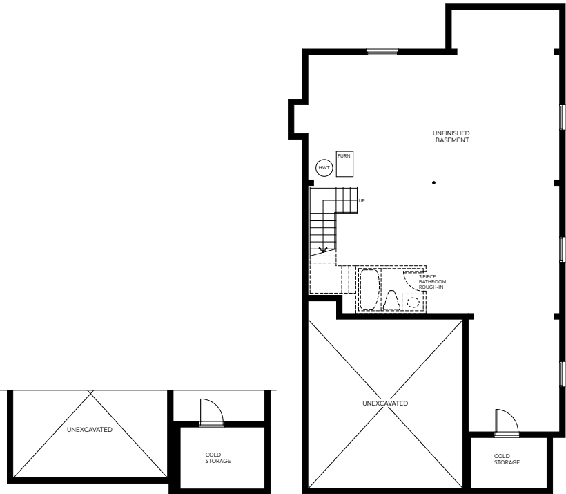
BASEMENT ELEVATION B
