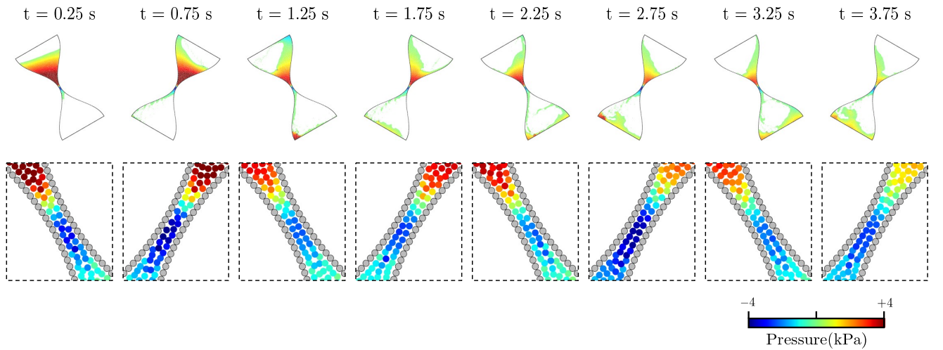
Fig.5.12: Pressure field contours of the entire hourglass and the constricted section
