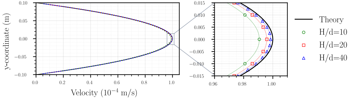
Fig.5.2: Velocity distribution at t = 1.00 s
