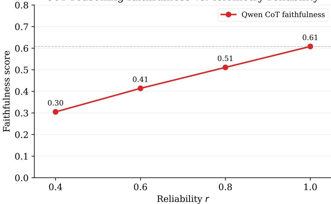
CoT reasoning faithfulness vs. telemetry reliability
