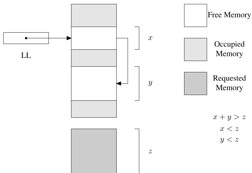
Fig. 5.11 External fragmentation
