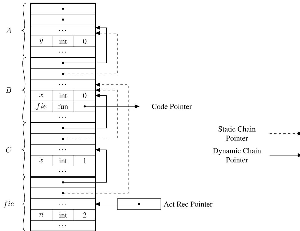
Fig. 5.12 Activation stack with static chain (see Example 5.3)
