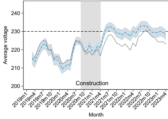
Figure A11: Impacts of transformer injection intervention on power quality and reliability
