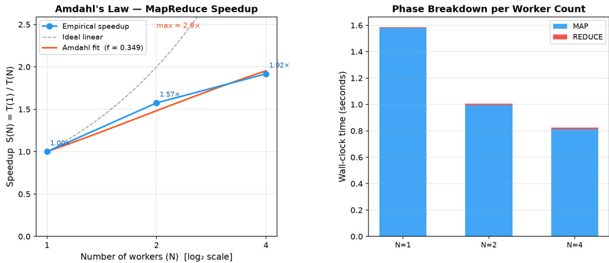
Figure 4: Single-machine Amdahl’s law. The fitted f = 0.349 is larger than on the cluster: co-located worker processes share one machine’s memory bandwidth and disk, inflating the serial fraction and capping the ceiling near 2.9\times . This contrast between the two figures is itself the lesson, Amdahl’s f is a property of the whole system , not just the algorithm.
