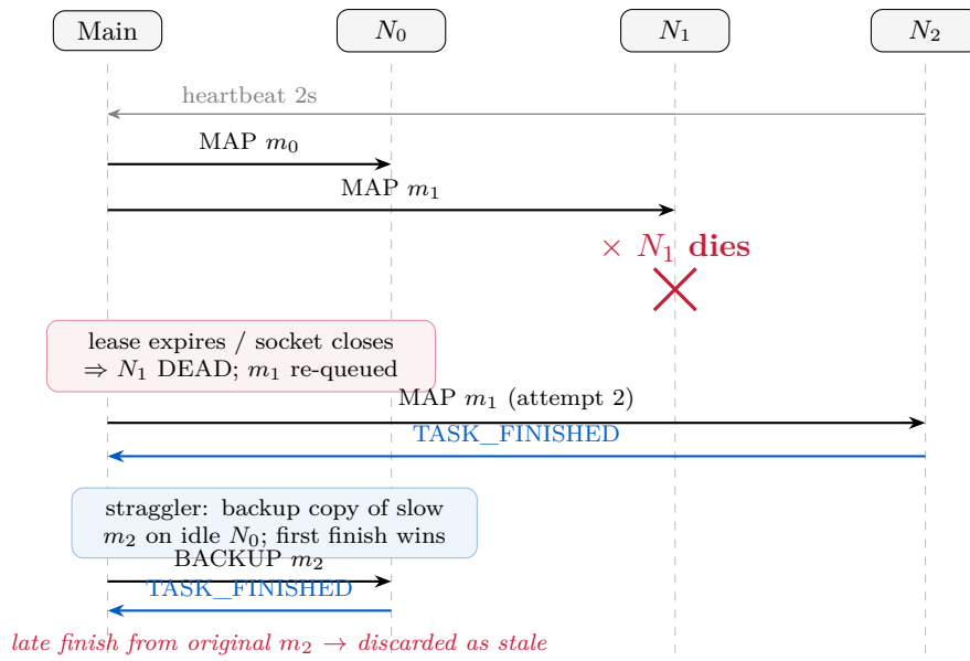
Figure 5: Fault-tolerance protocol (V2), simplified. Heartbeats feed a lease-based detector; a dead worker’s in-progress and completed-MAP tasks are re-executed; stragglers get backup copies. Full source: doc/fault_tolerance/fault_tolerance.secdiag.txt .
