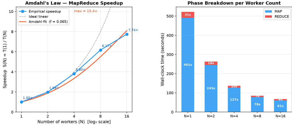
Figure 3: Cluster Amdahl’s law. Left: measured speedup vs ideal-linear, with a fitted serial fraction f = 0.065 implying a theoretical ceiling of \approx 15.4\times . Right: per-worker-count wall-clock split into MAP (blue) and REDUCE (red), showing MAP dominates and shrinks near-linearly with N .
