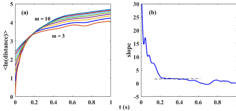
Fig. 7. LLE estimation: (a) Typical plot of the average exponential divergence versus time for embedding dimension m=3, \dots, 10 ; (b) slope corresponding to m=4 .
