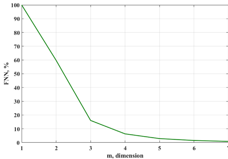
Fig. 2. Estimation of the gPPG minimum embedding dimension by the false nearest neighbors (FNN) method.
