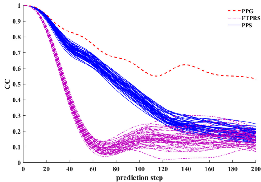
Fig. 5. Typical example of the CC between original and predicted time series for the gPPG (the red dashed line) and its 50 datasets of Fourier transform phase randomized (the purple dash-dotted lines) and pseudoperiodic (the blue lines) surrogates. (For interpretation of the references to color in this figure legend, the reader is referred to the web version of this article.)
