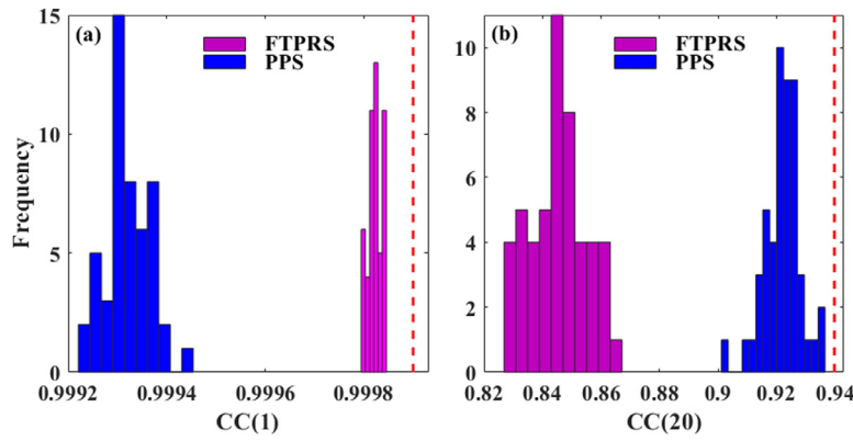
Fig. 6. Frequency distribution of correlation coefficient for 50 surrogate datasets of Fourier transform phase randomized (the purple bars) and pseudoperiodic (the blue bars) surrogates, and the corresponding correlation coefficient for original PPG signal (the red dashed line): (a) for 1 and (b) for 20 steps forward prediction. (For interpretation of the references to color in this figure legend, the reader is referred to the web version of this article.)
