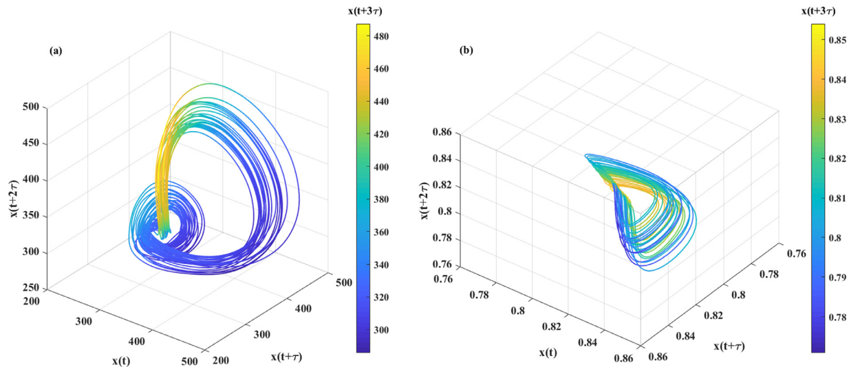
Fig. 3. Typical example of time-delay reconstructed trajectory with time-lag \tau = 40 for (a) gPPG and (b) rPPG.
