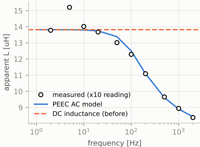
Claw-ZS: inductance vs frequency
