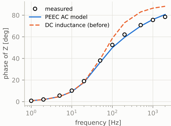
Claw-ZS: impedance phase (scale-free)
