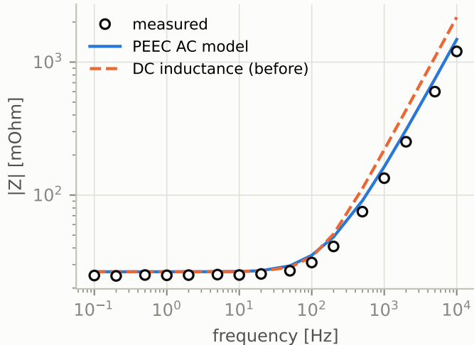
Olsen Bitter-ZS (held out): |Z(f)|
