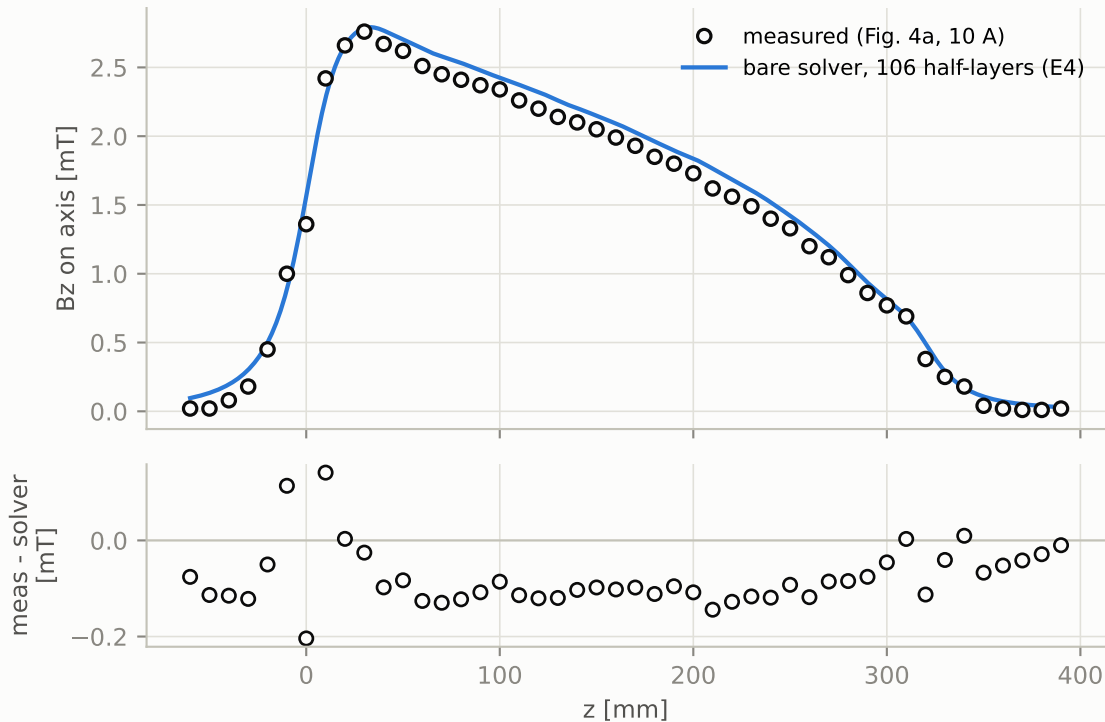
Claw-ZS (held out): axial field, nothing fitted
