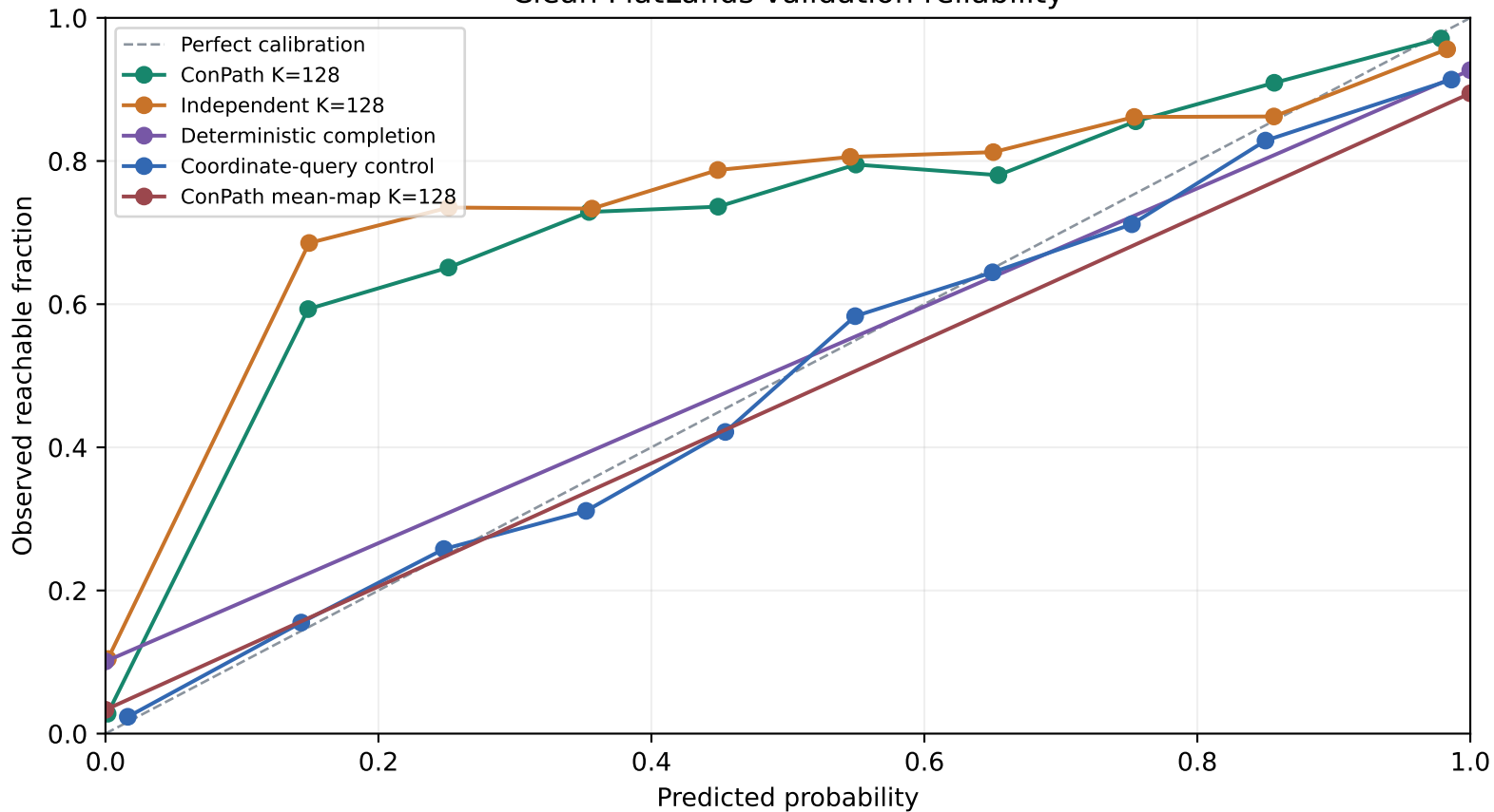
Clean FlatLands validation reliability
