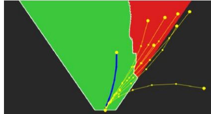
Selected (ours)
