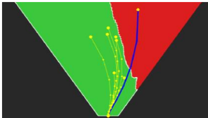
UnSelected
