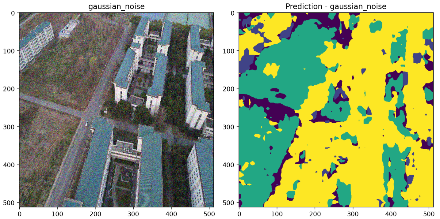
Gaussian Noise
