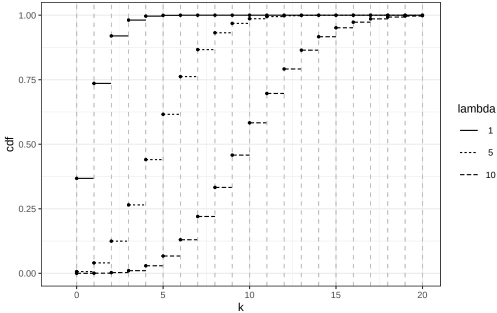
FIGURE 2.1 : Cumulative distribution functions for Poisson distributions with different parameters. Observe that, apparently, \mu \leq \nu \Rightarrow F_\mu \geq F_\nu . How would you establish this domination property?
