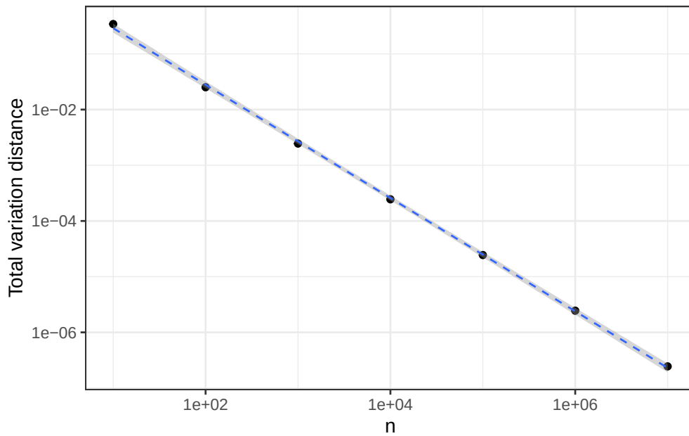
Figure 1.3: Law of rare events: distance between Binomial( n , 5/n ) and Poisson(5) as a function of n
